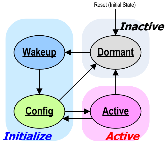
Figure 5-15 : Data Link State Machine (DLSM)
