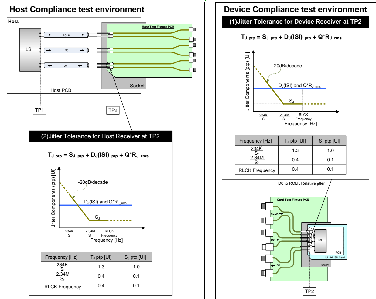
Figure 4-7: Jitter Tolerance Specification Notes of Figure 4-7 is a blank in the Simplified Addendum.
