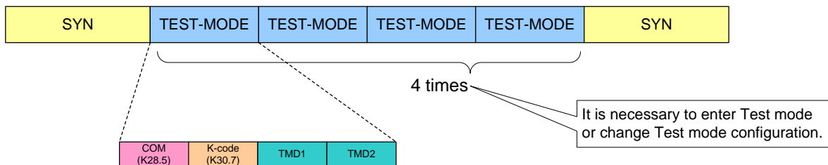
Figure 4-19: Sequences used in PHY Test Mode
