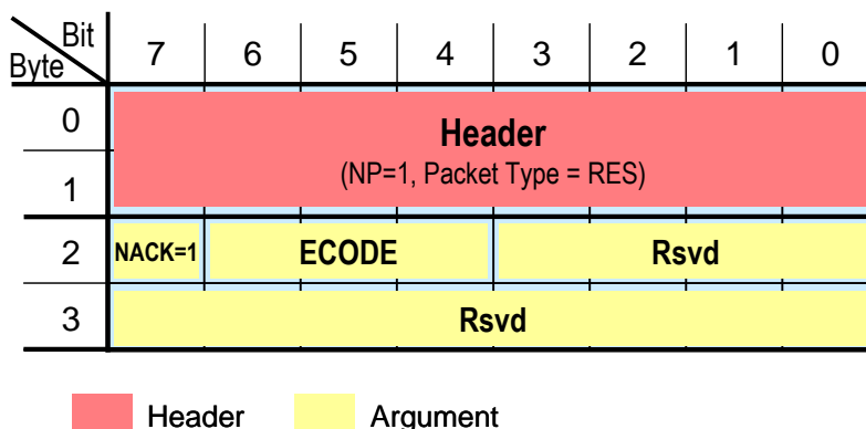
Figure 6-13 : RES (NACK = 1) Format
