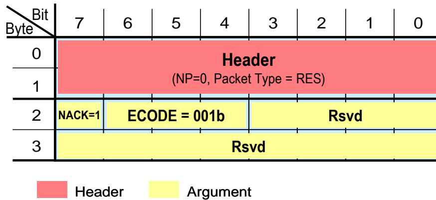
Figure 7-9 : RES (NACK = 1) Format on SD-TRAN
