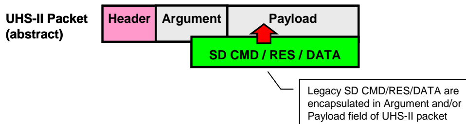
Figure 7-2 : Conceptual Diagram of SD-encapsulation
