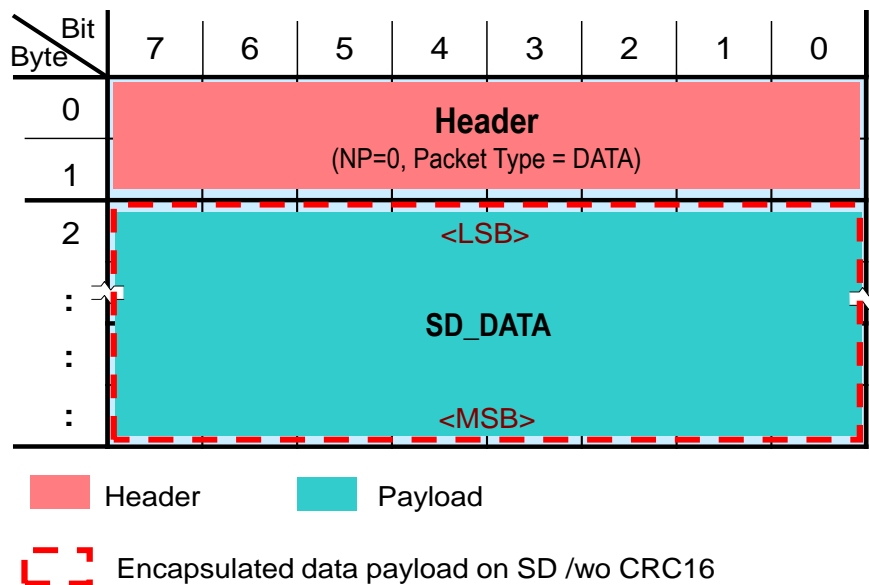
Figure 7-10 : DATA Format on SD-TRAN
