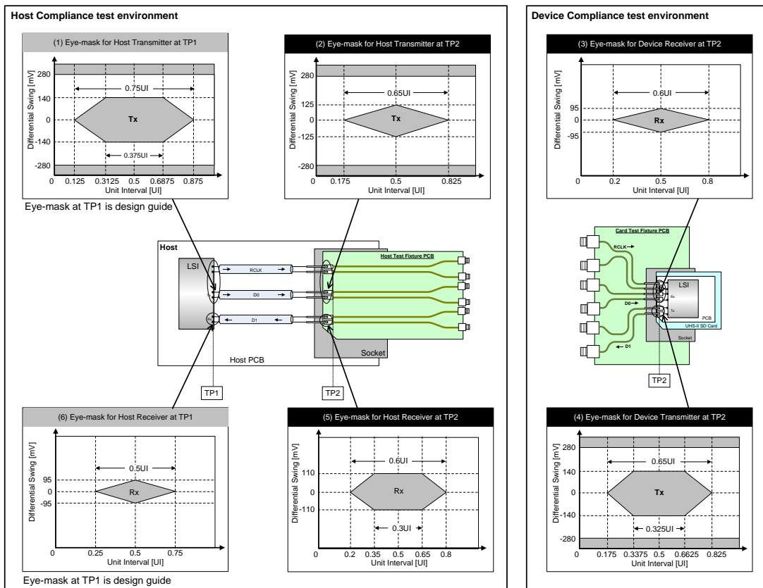
Figure 4-6: Eye-mask Templates
