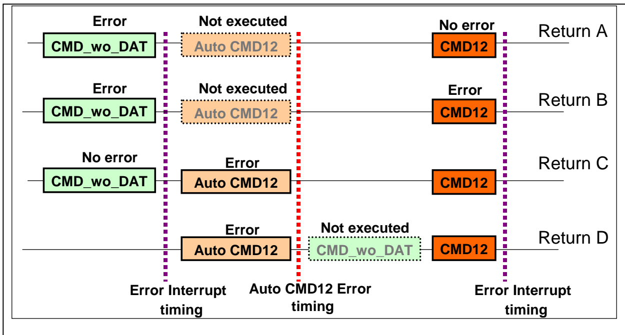
Figure 3-20: Return Status of Auto CMD12 Error Recovery
