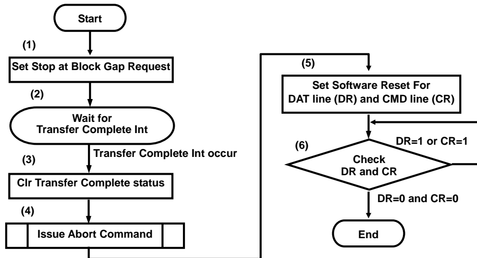
Figure 3-17: Synchronous Abort Sequence
