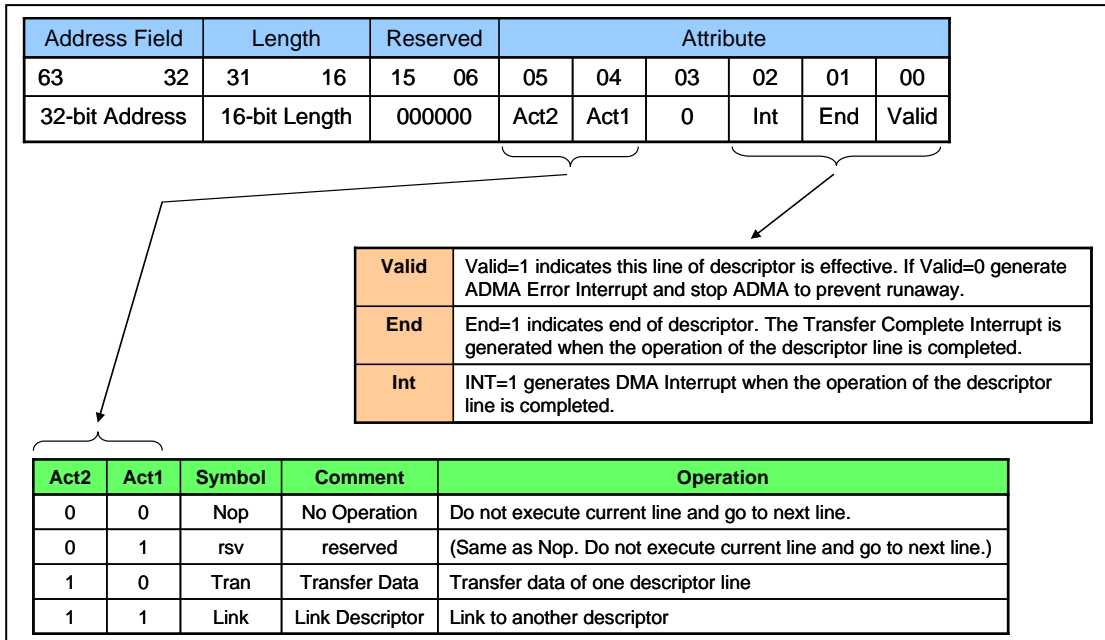
Figure 1-10 : 32-bit Address Descriptor Table
