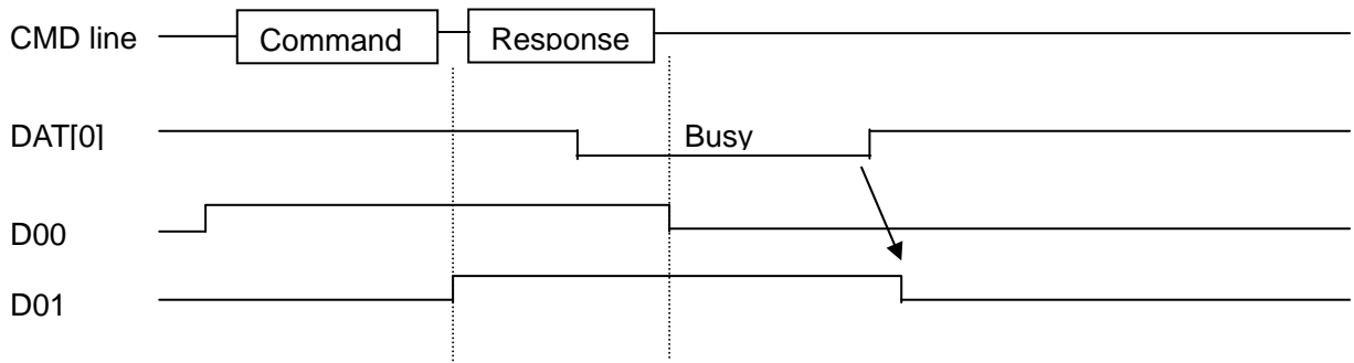
Figure 2-12 : Timing of Command Inhibit (DAT) for the Case of Response with Busy
