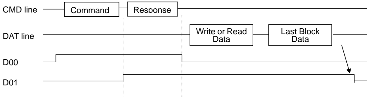
Figure 2-11 : Timing of Command Inhibit (DAT) and Command Inhibit (CMD) with Data Transfer
