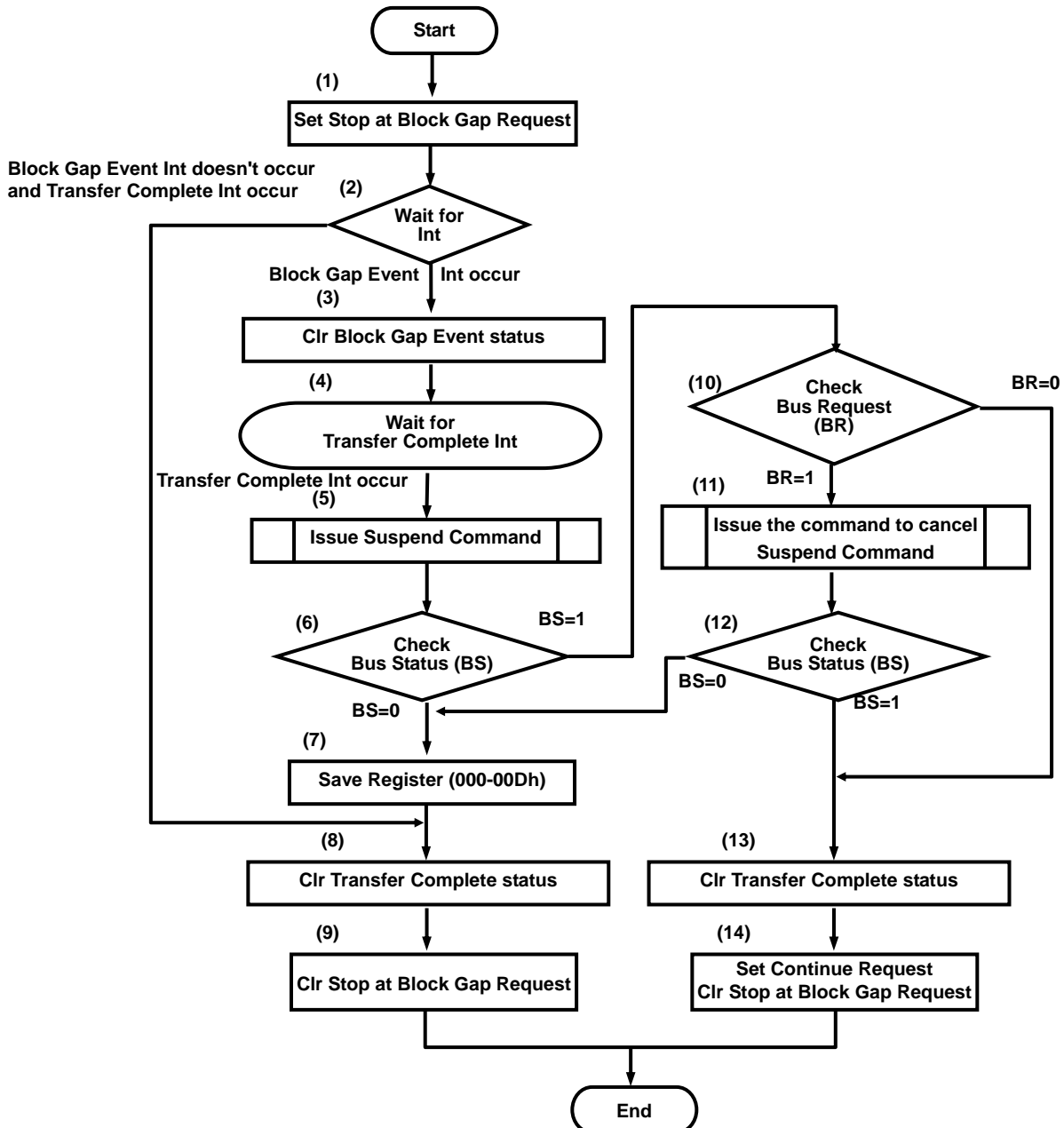
Figure 3-25 : The Sequence for Suspend
