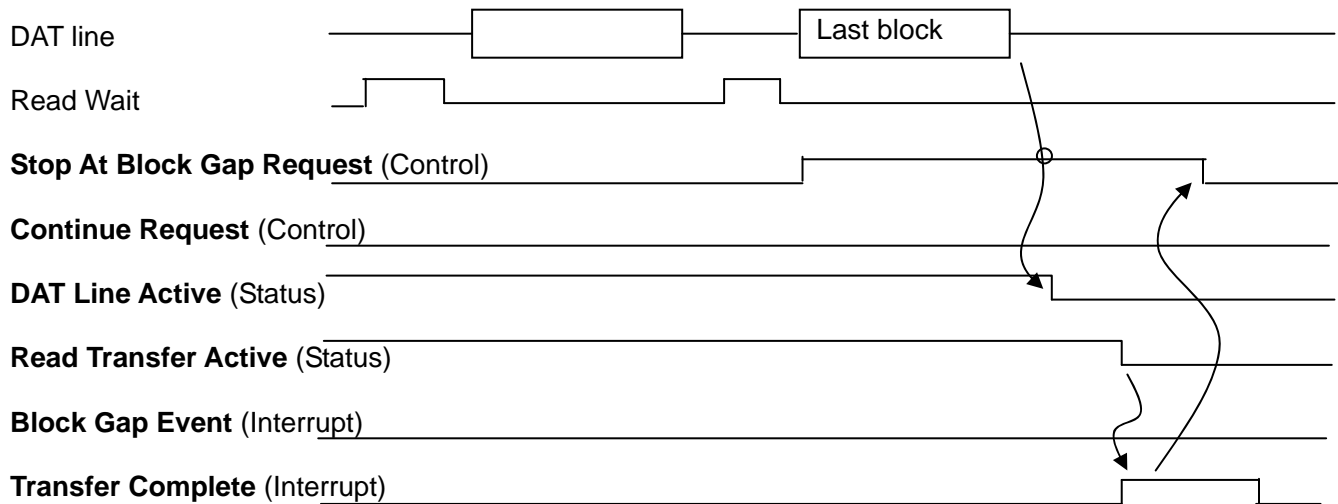
Figure 3-28 : Stop At Block Gap Request is Not Accepted at the Last Block of the Read Transfer
