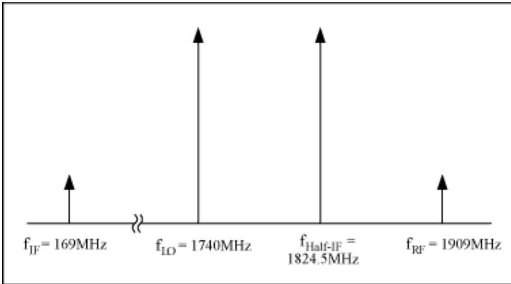
Figure 4. Frequency locations for desired f_{\text{RF}} , f_{\text{LO}} , f_{\text{IF}} , and undesired f_{\text{Half-IF}} .
