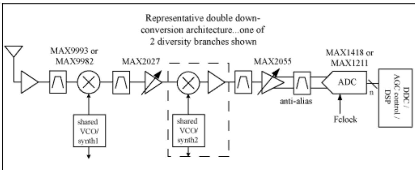
Figure 1. Subsampling receiver architecture.
